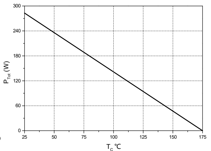
Figure 6. Power Derating
