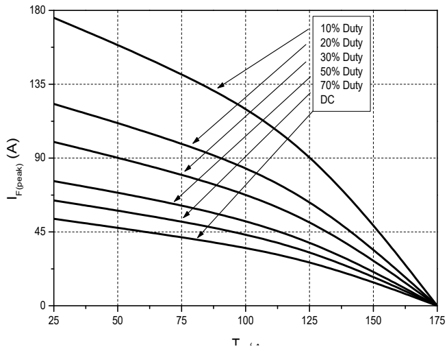
Figure 7. Current Derating
