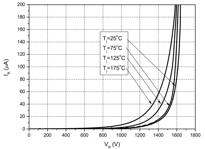
2. Reverse Characteristics
