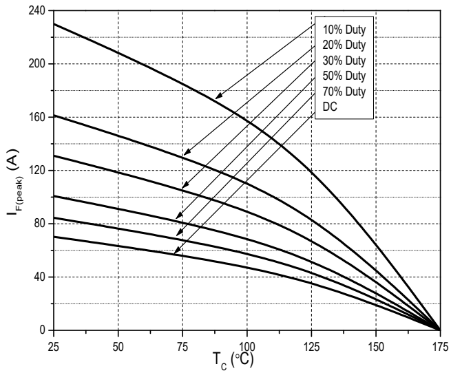
Figure 7. Current Derating
