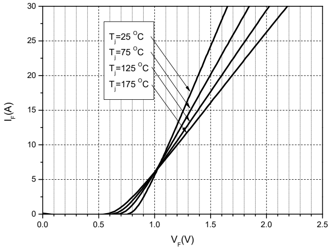
Figure 1. Forward Characteristics
