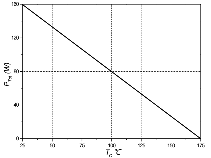
Figure 6. Power Derating
