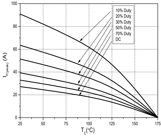
Figure 7. Current Derating
