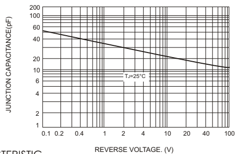
FIG.4-TYPICAL JUNCTION CAPACITANCE
